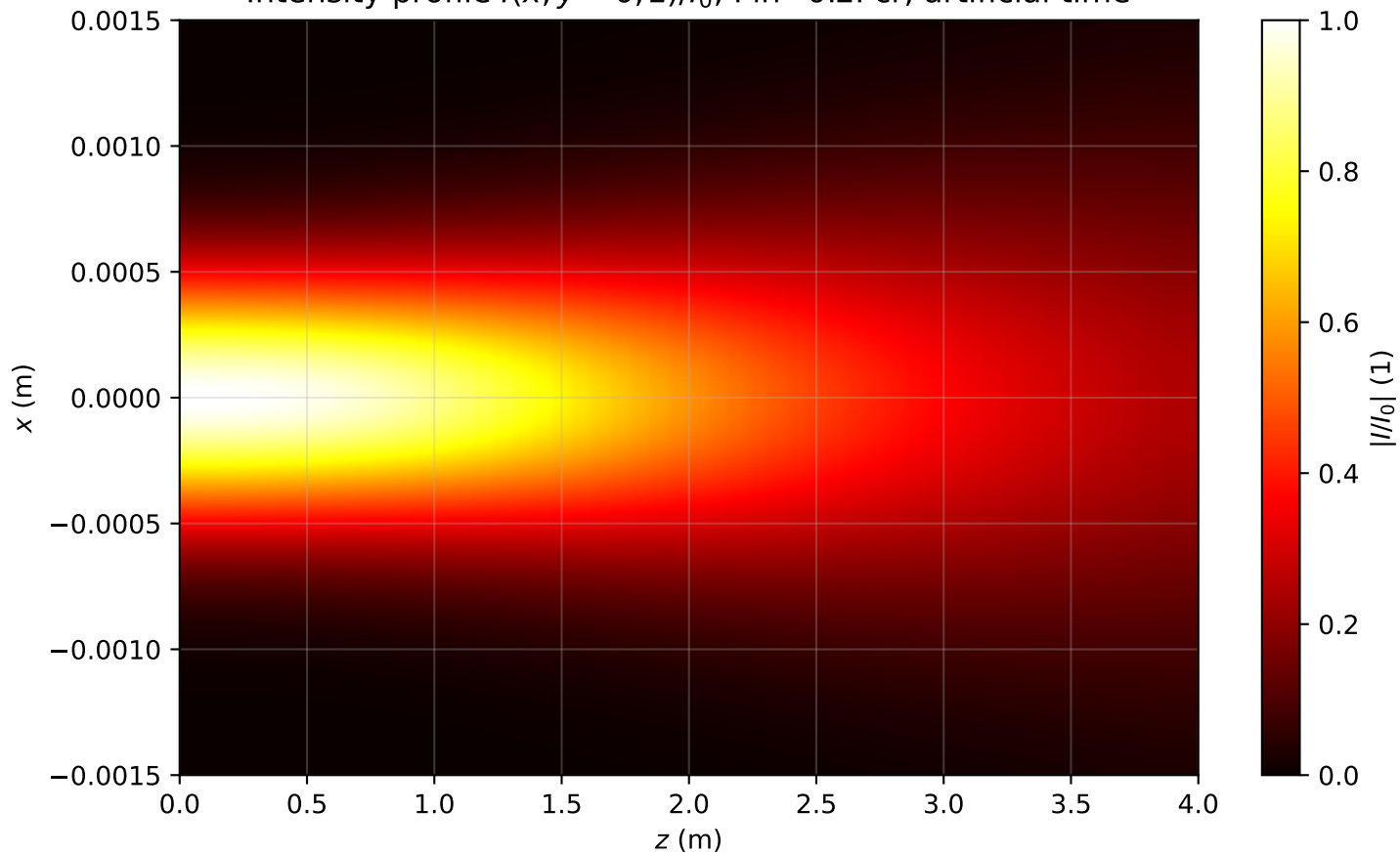
Intensity profile I(x, y = 0, z)/I_0 , P_{in}=0.2P_{cr} , artificial time
